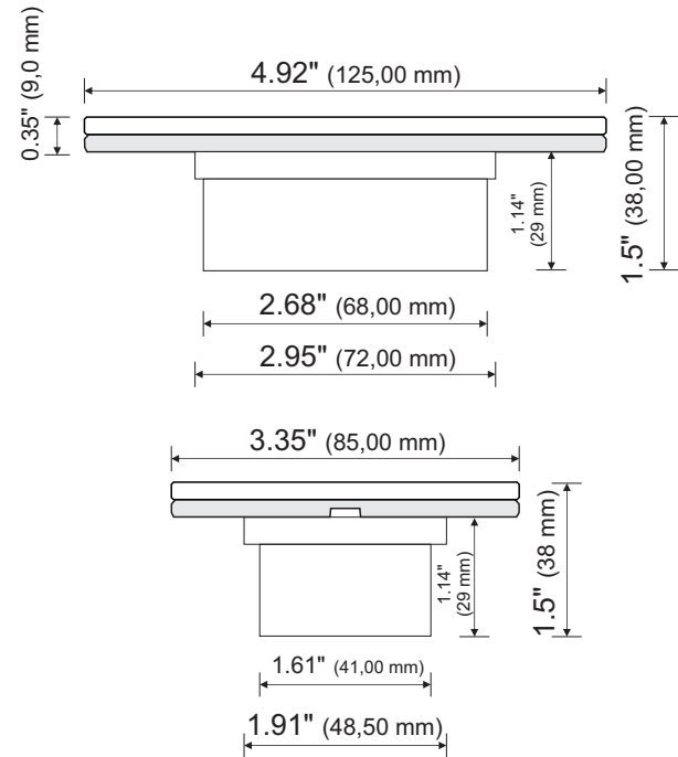
Scale 1:2 (dimensions are in inch (mm))
